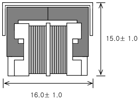
3) SIDE VIEW
